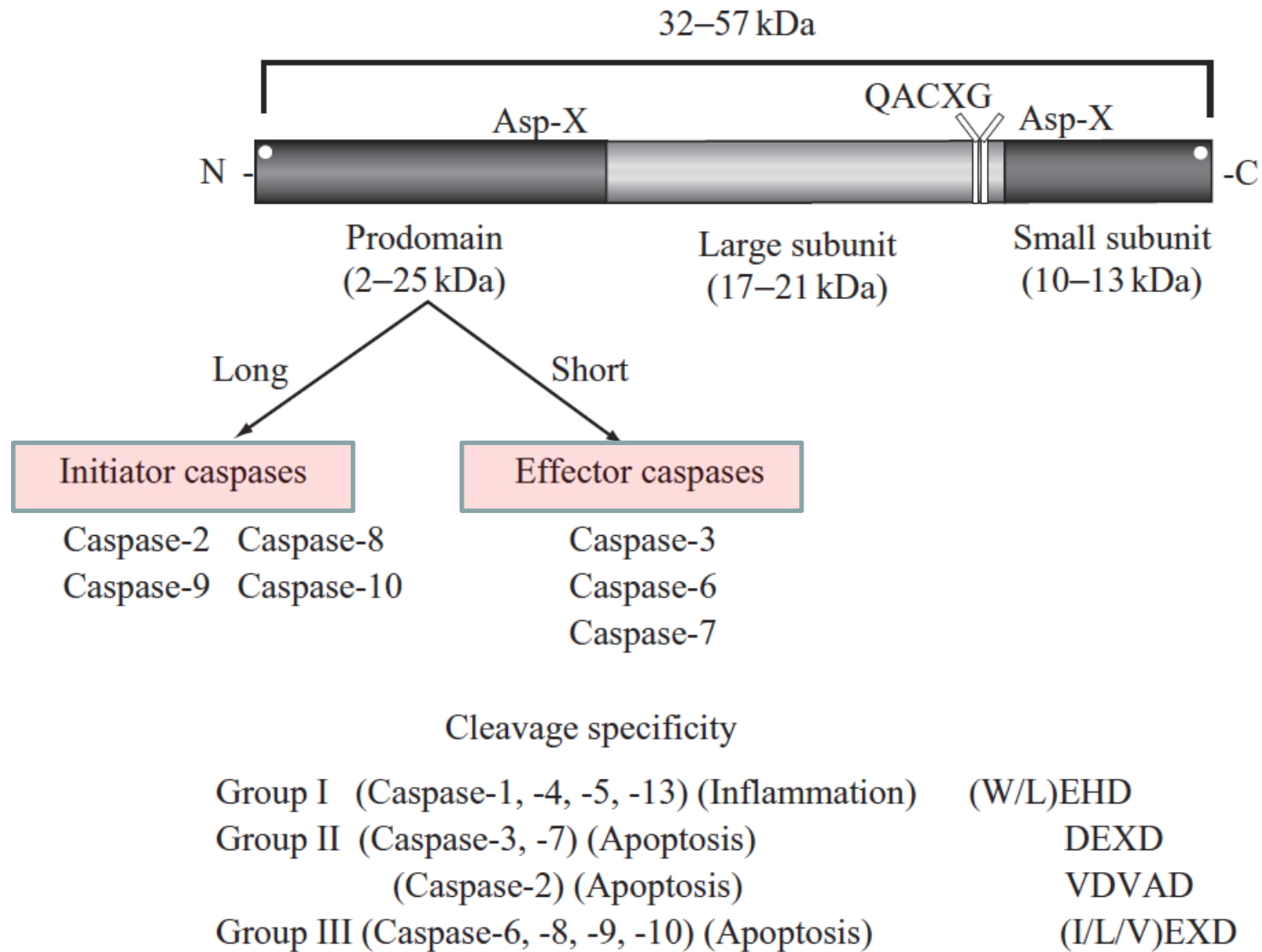
Figure 8.2 The structural and functional organization of caspases.
