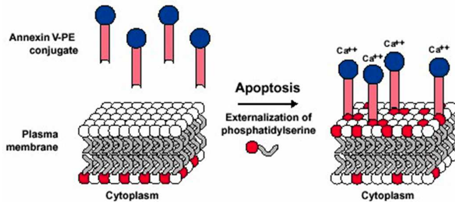
Schematic representation of the Annexin V assay.
