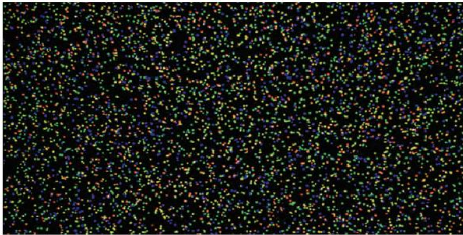
A slide showing individual clusters of PCR-generated DNA molecules. Each cluster carries about 1000 identical DNA molecules; the four colors are produced by incorporation of C, G, A, or T, each of which has a different color fluorophore. The image has been taken just after a fluorescent nucleotide has been incorporated into each growing DNA chain. (From Illumina Sequencing Overview, 2013.)
