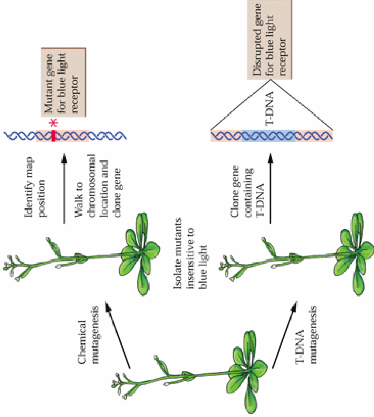
(A) Chemical mutagenesis vs. T-DNA mutagenesis
