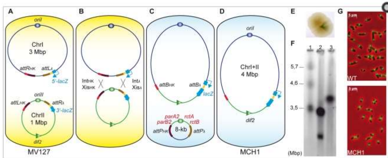
A mono-chromosomal V. cholerae model, MCH1.
