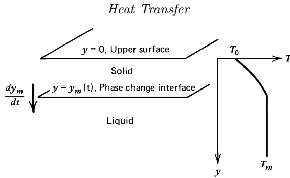
Figure 4.29 Growth of a solid layer at the surface of a cooling lava flow.
