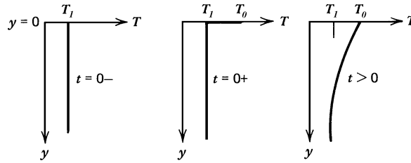
Figure 4.20 Heating of a semi-infinite half-space by a sudden increase in surface temperature.
