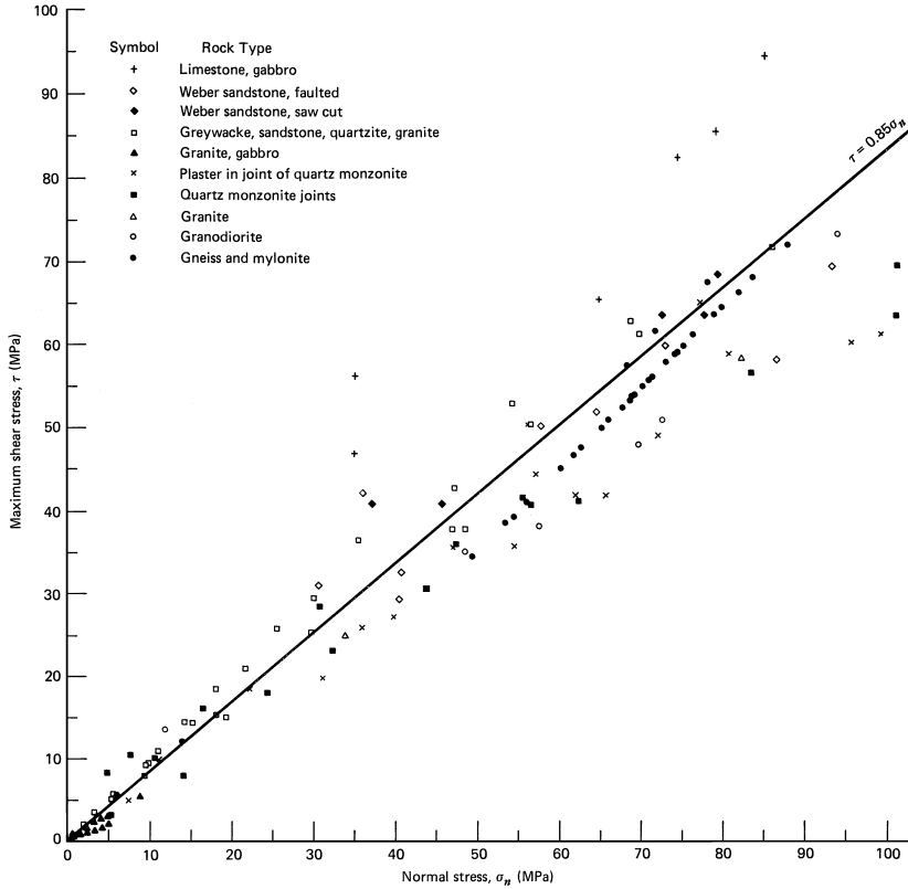
Figure 8.7 Maximum shear stress to initiate sliding as a function of normal stress for a variety of rock types. The linear fit defines a maximum coefficient of static friction \max f_s equal to 0.85. Data from Byerlee (1977).
