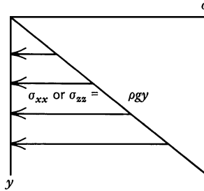
Figure 2.9 The area under the stress versus depth profile is proportional to the total horizontal force on a vertical plane.
