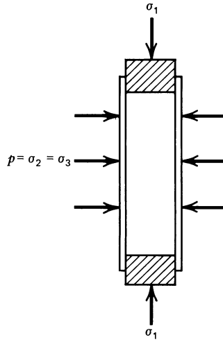
Figure 3.6 Sketch of a triaxial compression test on a cylindrical rock sample.
