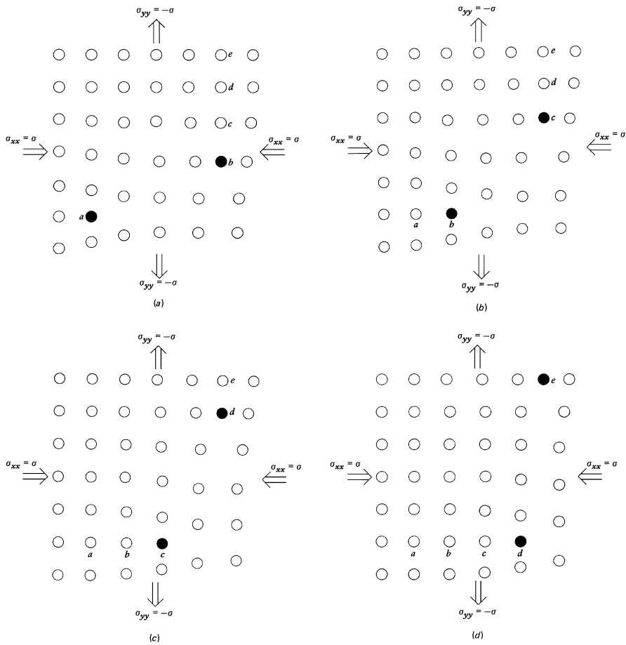
Figure 7.11 The process of dislocation climb. Because of the diffusion of the atoms b , c , and d from the extra vertical plane of atoms to the additional horizontal plane of atoms, the crystal is shortened in the x direction and lengthened in the y direction. This is the result of the tensional stress in the y direction and the compressional stress in the x direction that drives the diffusion of atoms between the two dislocations.
