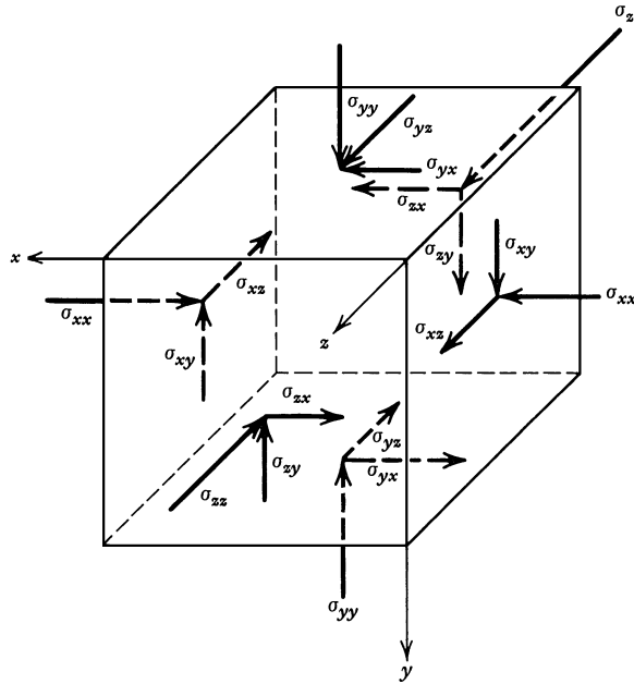
Figure 2.15 Stress components on the faces of a small rectangular parallelepiped.
