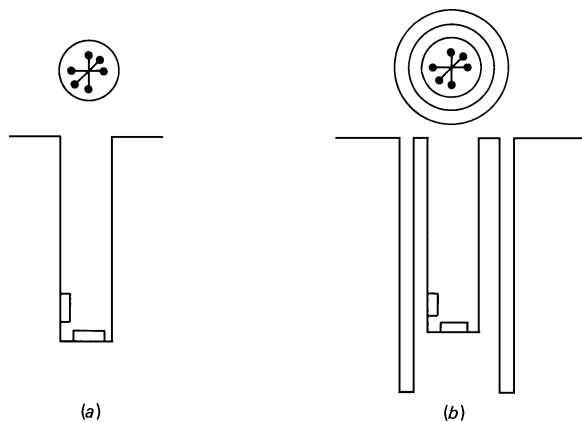
Figure 2.17 Schematic of overcoring technique for stress measurements. (a) A hole is drilled, and four strain gauges are installed: one on the side wall to measure \sigma_{yy} and three on the base to measure \sigma_{xx} , \sigma_{xz} , and \sigma_{zz} . It is assumed that the drilling of the hole has not affected the ambient state of stress. (b) The second annular hole is drilled. It is assumed that this annular hole completely relieves the initial stresses.
