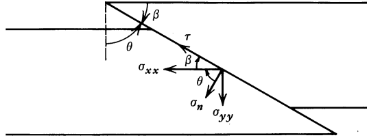
Figure 8.8 Principal stresses and normal and tangential stresses on a dip-slip fault.
