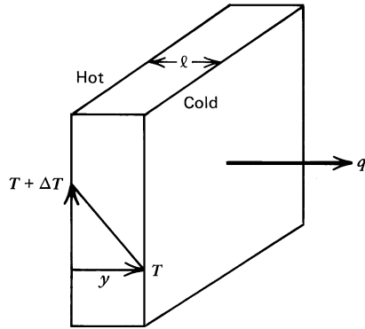
Figure 4.1 Heat transfer through a slab.
