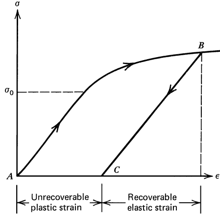
Figure 7.27 Stress-strain history for loading and unloading of an elastic-plastic material.
