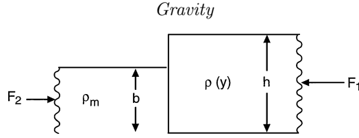
Figure 5.23 Force balance on a section of continental crust and lithosphere.
