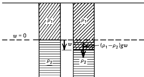
Figure 6.22 The buoyancy force associated with the displacement of the interface.
