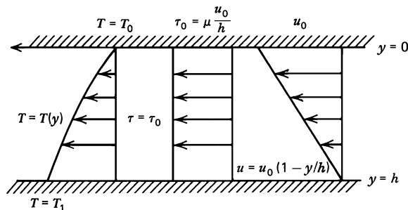
Figure 6.45 Frictional heating in Couette flow.
