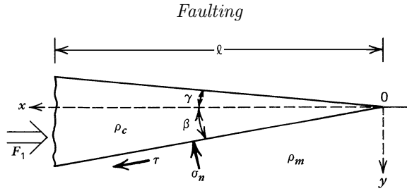
Figure 8.14 A wedge-shaped model of a thrust sheet.
