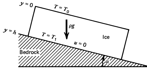
Figure 7.16 An ice sheet of thickness h on bedrock sloping at angle \alpha . The ice will creep downhill under its own weight.
