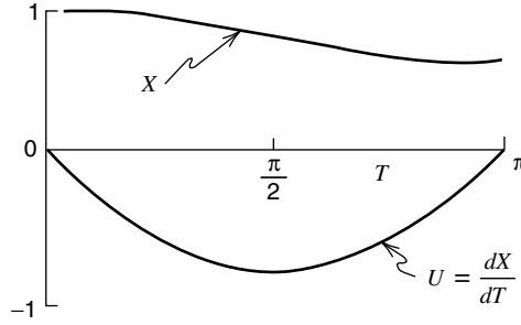
Figure 8.19 Dependence of the nondimensional slider-block position X and velocity dX/dT on time T during a slip event as given by Equations (8-64) and (8-65) for \phi = 1.25 .
