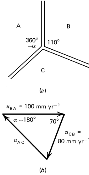
Figure 1.36 (a) Schematic of a ridge–ridge–ridge (RRR) triple junction of plates A, B, and C. (b) Vector velocities for relative motion between the plates.
