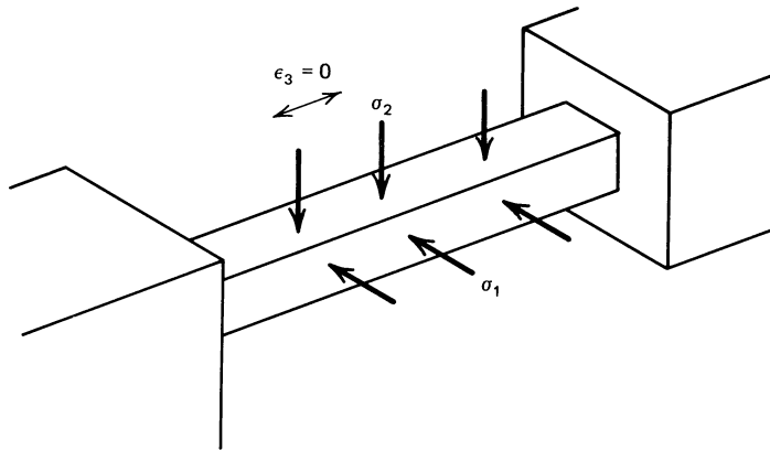
Figure 3.7 An example of plane strain.
