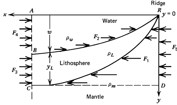
Figure 6.44 Horizontal forces acting on a section of the ocean, lithosphere, and mantle at an ocean ridge.
