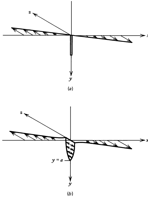
Figure 8.25 The displacement field due to faulting on a model strike-slip fault. The surface is at y = 0 and the fault is at x = 0 , 0 \leq y \leq a . Displacements are in the z direction. (a) Initially the half-space y > 0 is in a state of uniform shear stress \sigma_{xz,0} . (b) After the introduction of the crack the shear stress on the crack is zero ( \sigma_{xz} = 0 ) and there is a displacement across the crack.
