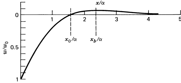
Figure 3.32 The deflection of the elastic lithosphere under an end load.
