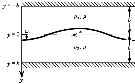
Figure 6.21 The Rayleigh–Taylor instability of a dense fluid overlying a lighter fluid.
