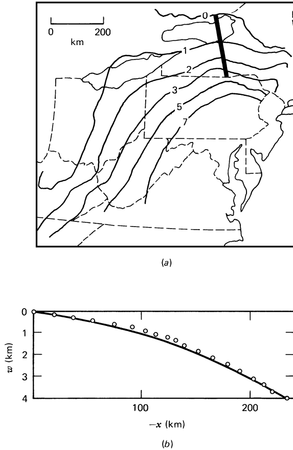
Figure 3.36 (a) Contours of basement (in km) in the Appalachian basin of the eastern United States. Data are from well logs and seismic reflection studies. (b) The data points are the depths of basement below sea level as a function of the distance from the point where basement rocks are exposed at the surface along the profile given by the heavy line in (a). The solid line is the universal flexure profile from Equation (3-159) with x_b = 122 km and w_b = 290 m ( x_0 = 0 ).
