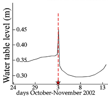
Figure 3. Examples of water changes during earthquakes. The L'Aquila-Italy, 2009 normal fault example illustrates an increase in water supply at a spring 14 km from the epicenter (Gran Sasso-Assergi) that began slowly days before the main event. An upraise of the water table was described during the Borah Peak-Idaho, 1983 normal fault-related earthquake. The thrust fault example (Northridge, 1994) shows a typical pattern of both lowering and upraising of the water table or discharge at springs. Along strike-slip faults a similar pattern occurs, with both uplift and lowering of the water level as evident for the Denali, 2002 event. The cross-sections to the right qualitatively illustrate the location of measurement with respect to the fault. In the strike-slip example, the rectangle simplifies the activated subvertical dextral strike-slip fault plane, and the water variations are in the eastern wall of the fault. Data of the L'Aquila 2009 event after courtesy of Gran Sasso S.p.A. Bora Peak Whitehead et al. (1985) , Northridge, Sneed et al. (2003) , Denali, Sil (2006) .
