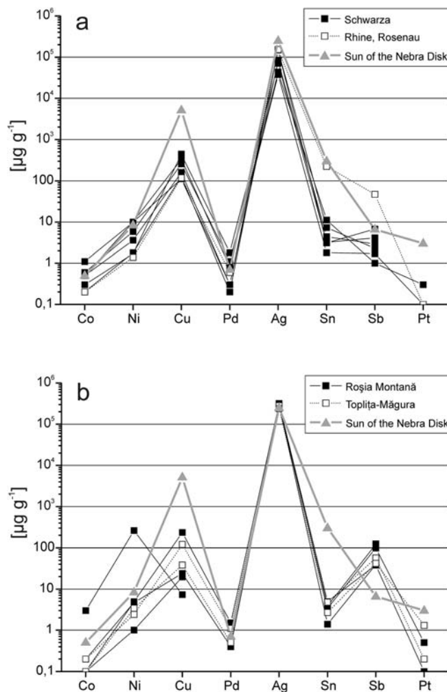
Fig. 4. Minor and trace element concentrations (median) of the gold occurrences in central (a) and southeastern (b) Europe that result from cluster analysis by Schmiderer (2009), in comparison with the composition of the gold from the sun sheet of the Nebra Sky Disk (grey triangle).
