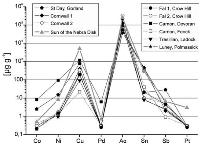
Fig. 5. Minor and trace element concentrations (median) of the Cornish gold occurrences in comparison with the composition of the gold from the sun sheet of the Nebra Sky Disk (grey triangle).
