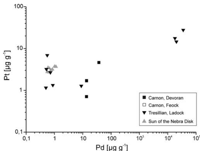
Fig. 3. Pt and Pd concentrations of the Cornish gold occurrences in comparison with the concentrations of the gold from the sun sheet of the Nebra Sky Disk (grey triangle).
