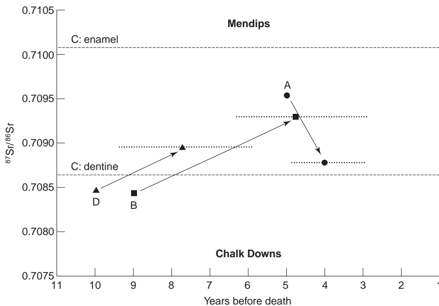
Figure 3. Strontium isotope ratios for the juveniles' tooth enamel relative to its time of formation in years before death. Error bars associated with the permanent teeth represent the maximum period of enamel mineralization. The adult female, C, is represented by dashed lines indicating the values of her enamel and dentine.
