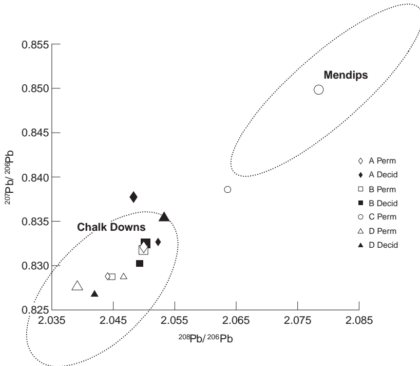
Figure 2. Lead isotope ratios for the deciduous and permanent tooth enamel (large symbols) and dentine (small symbols) of the three juveniles (A, B and D) and permanent tooth enamel and dentine for the adult female (C). Errors on the Pb isotope ratios were determined from replicate analysis of the NBS 981 standard as 0.014% for ^{207}\text{Pb}/^{206}\text{Pb} and 0.024% for the ^{208}\text{Pb}/^{206}\text{Pb} ( n = 27, 2\sigma ). These are smaller than the symbols at this scale.
