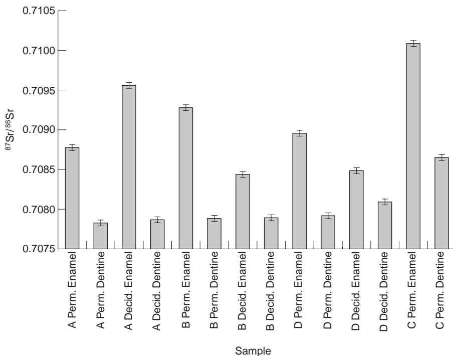
Figure 1. Strontium isotope ratios for the deciduous and permanent tooth enamel and dentine of the three juveniles (A, B and D) and permanent tooth enamel and dentine for the adult female (C). Error bars represent 2\sigma errors calculated from 10 replicates of the NBS 987 standard.
