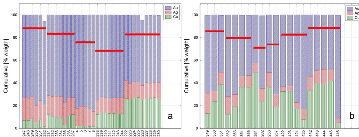
Fig. 8. a. Elemental composition of five objects showing internal homogeneity and inter object variability. b. Elemental composition of six objects taken in different points, showing internal variability.
