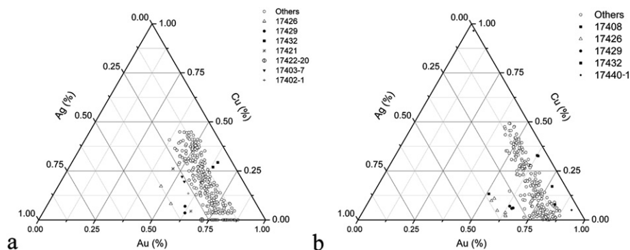
Fig. 7. Ternary diagrams showing Au–Cu–Ag compositions for all measures, where three main groups of objects are identified: a. XRF results (287 data points from all 135 Quimbaya items). b. PIXE results (242 data points from 63 Quimbaya items).
