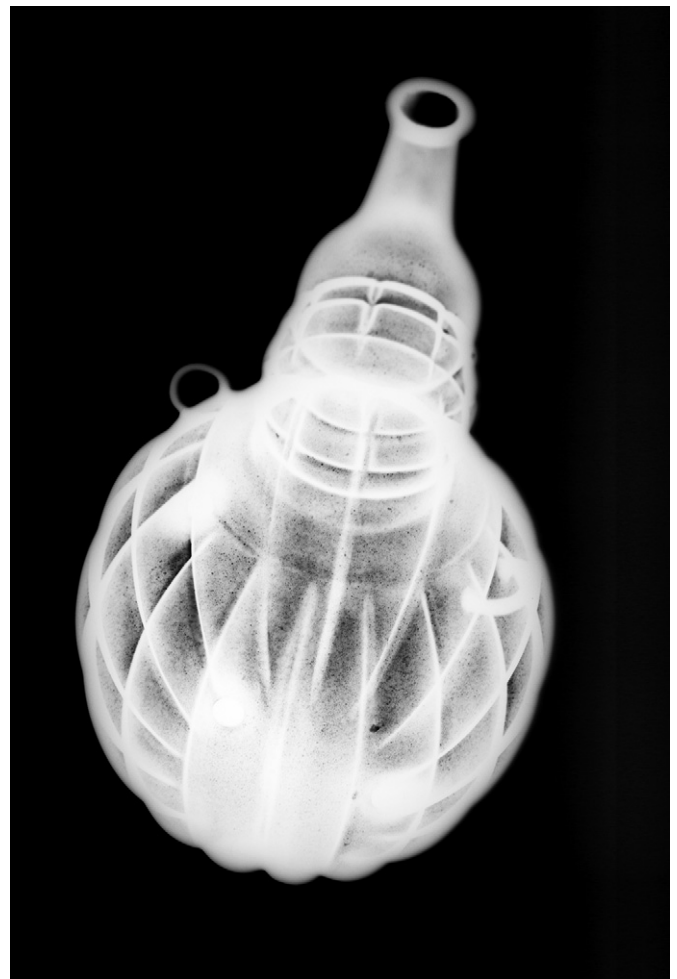
Fig. 11. X-ray image of a phytomorphic vessel showing the perfect modelling of the wax, and fine and homogeneous porosity (darker spots). Museo de América, Madrid (photo: Archivo Gabaldón-Antelo, IPCE).
