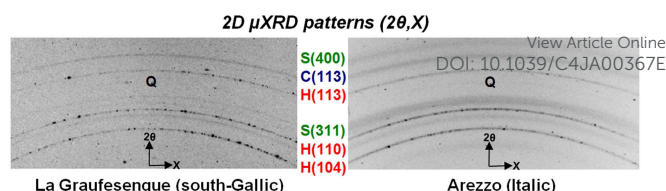
Fig. 3 2D \mu\text{XRD} patterns obtained in the slip of south-Gallic and Italic sigillata samples ( 2 \times 3 \mu\text{m}^2 beam) (H: Hematite, S: Spinel, C: Corundum and Q: Quartz).
