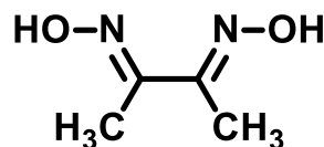
Diacetildiossima
