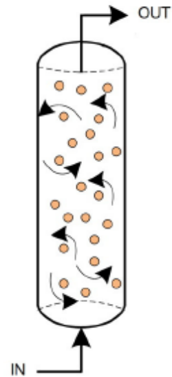
FLUIDIZED-BED REACTOR
