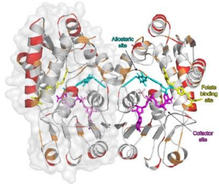
Figure 8. Structure of the hMTHFD2L dimer highlighting the three different ligand binding sites. The surface of one monomer is shown at 80 % transparency. The structure was superimposed with that of MTHFD2–TH7299 (PDB ID: 6S4E) and MTHFD2–J4C (PDB ID: 7EHM), however only the ligands of the compared structures are shown. TH7299 which binds in the MTHFD2L folate binding site is shown as yellow sticks. Partial NADP + (MTHFD2L) and NAD + (MTHFD2) which bind in the cofactor binding site are shown as light pink and magenta sticks, respectively. The allosteric inhibitor J4C (MTHFD2) is shown as cyan sticks. Amino acid differences between MTHFD2L and MTHFD2 are highlighted. Red coloring indicates non-conserved differences and orange coloring indicates differences with conserved physicochemical properties. Figures were produced with PyMOL (v.2.3.3, Schrödinger).
