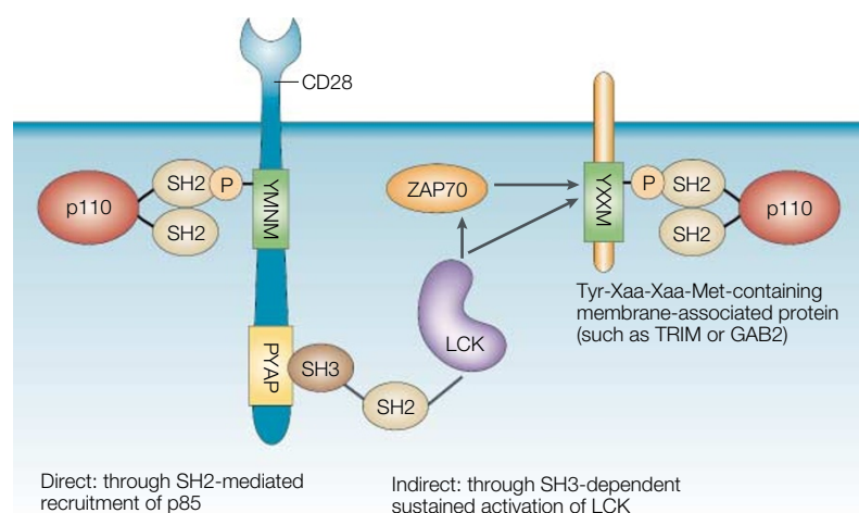
Figure 4 | Two modes of CD28-dependent activation of PI3K. In the direct mode, the p85 SRC-homology 2 (SH2) domains bind the phosphorylated Tyr-Met-Asn-Met (YMNM) motif in the cytoplasmic domain of CD28 (REF. 106). This is analogous to the manner in which growth-factor receptors, such as platelet-derived growth factor receptor and c-KIT, recruit and activate class IA phosphoinositide 3-kinases (PI3Ks). The second mode of activation is more speculative at this time, and is based on the observation that the proline-rich region of CD28 (PYAP) is required for CD28 to sustain LCK in its activated state (the initial activation is controlled by the TCR and CD4) 115,121 . The link between LCK and PI3K could involve the phosphorylation of TCR-interacting molecule (TRIM; a transmembrane adaptor protein with Tyr-Xaa-Xaa-Met, YXXM, motifs), linker for activation of T cells (LAT; which lacks Tyr-Xaa-Xaa-Met motifs, but which might couple to PI3K indirectly through GAB) or other linker proteins with Tyr-Xaa-Xaa-Met motifs. LCK could phosphorylate these targets directly or through its activation of \zeta -chain-associated protein kinase 70 kDa (ZAP70). Either way, CD28 could contribute to T-cell-receptor-dependent PI3K activation by virtue of its capacity to influence the kinetics of LCK activation.
