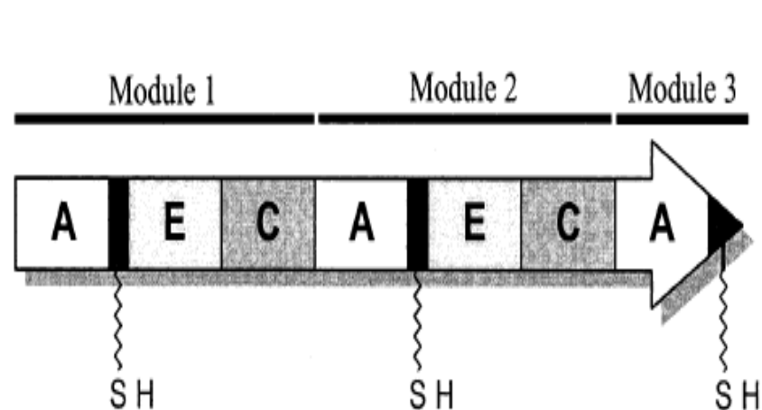
Fig. 1. Domain and module organization of the NRPS (CchH) encoded on cosmid SCF-34 of the ordered S. coelicolor genomic library. Domains are indicated as follows: adenylation: A, white; PCP: black, ~SH; epimerization: E, light gray; and condensation: C, dark gray.
