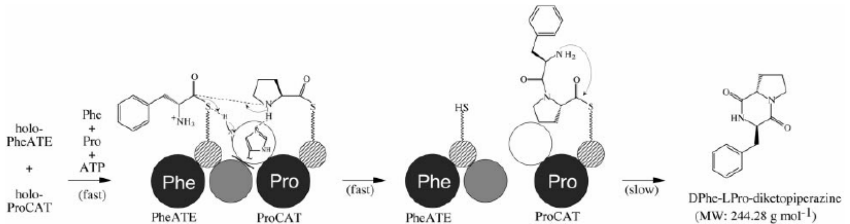
FIG. 7. Reaction sequence of D-Phe-L-Pro and diketopiperazine formation. A proposed simple model for peptide bond and diketopiperazine formation is shown. The single domains of the modules PheATE and ProCAT are illustrated as black (adenylation), striped (thiolation), gray (epimerization), and white (condensation) circles. PheATE and ProCAT are loaded with their cognate amino acids. His 147 of ProCAT, a strictly conserved residue of the condensation domain, acts as a base to promote the nucleophilic attack of the imino group of L-Pro onto the carboxy carbon atom of D-Phe. Another residue should reprotonate the thiol moiety of the liberated P-pant. The black line indicates protein-protein interactions between ProCAT and the C-terminal region of PheATE. In a second step, diketopiperazine formation is believed to occur by an intramolecular, noncatalyzed cyclization reaction.
