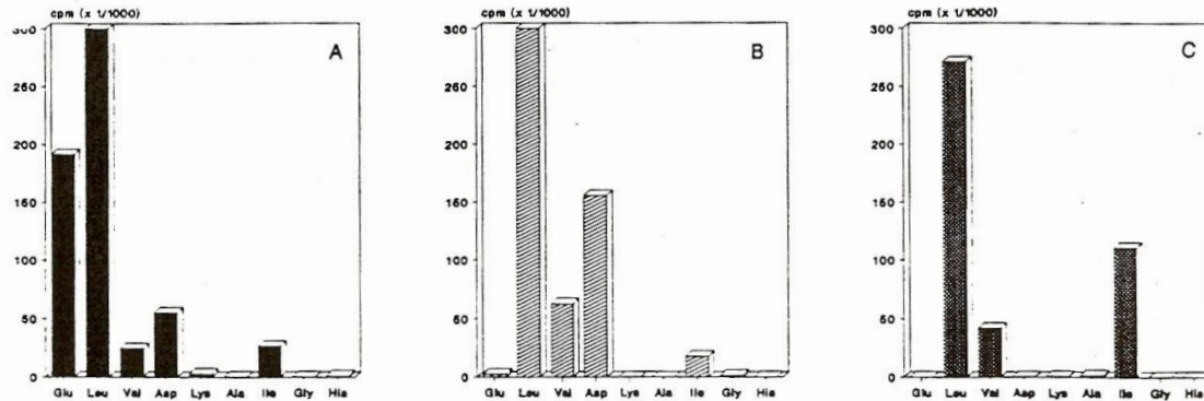
Fig. 4. ATP/PP i exchange activity of srfAORF1, srfAORF2 and srfAORF3. The partially purified subunits were incubated in the presence of ATP, [ 32 P]PP i and one amino acid and, after 10 min incubation at 37°C, the [ 32 P]ATP was adsorbed on Norite A (activated coal, Sigma) and counted.
