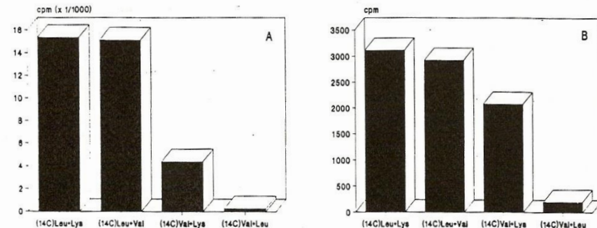
Fig. 6. Amino-acid binding competition experiments. Either srfAORF1 (A) or srfAORF3 (B) were incubated simultaneously with two amino acids, one of which [ 14 C]-labelled. Samples were processed as described in Fig. 5. See text for details.
