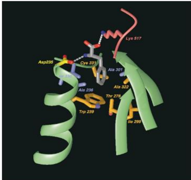
Figure 3. The Phenylalanine binding Pocket of PheA as a Prototype Substrate binding Pocket for the Superfamily of Adenylate-Forming Enzymes
