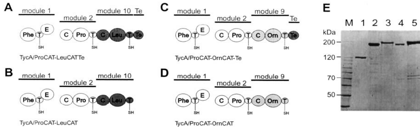
Fig. 3. Construction of artificial trimodular NRPS systems. Artificial trimodular NRPS systems were obtained by extension of the first two modules of tyrocidine synthetases, TycA and TycB1 (here referred to as ProCAT). Fusion of the last module of TycC, containing the Te-domain, to ProCAT yielded TycA/ProCAT-LeuCATTe (A). TycA/ProCAT-LeuCAT is devoid of the Te-domain (B). Fusion of the second last module of TycC, OrnCAT, resulted in the system TycA/ProCAT-OrnCAT (D), which was extended in a second fusion step to TycA/ProCAT-OrnCAT-Te (C). The purified His 6 -tagged enzymes are shown on a Coomassie blue-stained SDS/PAGE (7.5% polyacrylamide) in E. M = marker. Lanes 1–5: TycA, ProCAT-OrnCAT, ProCAT-OrnCAT-Te, ProCAT-LeuCAT, and ProCAT-LeuCATTe, respectively. The gel could not sufficiently resolve the dimodular enzymes, which are 234–265 kDa in size.
