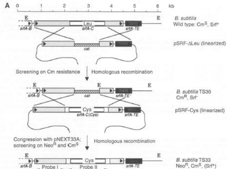
Fig. 3. Targeted srfA-C replacement in B. subtilis . (A) The integrative plasmids constructed (Fig. 2B) were used for in vivo srfA-C disruption and domain substitution within the chromosome of B. subtilis . Two steps were required: first, the srfA-C gene of B. subtilis (ATCC 21332) was disrupted by homologous recombination with the linearized plasmid pSRF- \Delta Leu (11). Subsequently, a domain substitution was achieved by a marker exchange reaction, mediated by the desired domain substitution plasmid (for instance, pSRF-Cys) bearing the gene of a hybrid synthetase (11). Loss of the cat cassette and the unlinked cotransformation (congression) with pNEXT33A, mediating neomycin resistance ( Neo^R ), were used to identify strains carrying domain replacements (11). Cleavage sites of the restriction enzyme Eco RI within the chromosomal location of srfA-C are shown (E). Cm^S , chloramphenicol-sensitive. (B) Southern blots of Eco RI-digested genomic DNA were probed with the 5'-linker fragment (left panel) and the substituted Cys domain-coding area of acvA (right panel) [shown as double-arrows in (A)], respectively (16). For a positive control, we used the unlabeled 5'- srfA-C fragment (left) and acvA (right) (lanes 1). Genomic DNA was prepared from the wild-type strain B. subtilis (ATCC 21332) (lanes 2), TS30 (lanes 3), and TS33 (lanes 4) [compare (A)]. Lanes 5 show Hind III-digested \lambda DNA as a negative control. The patterns confirmed the disruption (TS30) and domain exchange (TS33) by homologous integration, as shown above. Size markers are indicated on the sides of the gels in kilobases.
