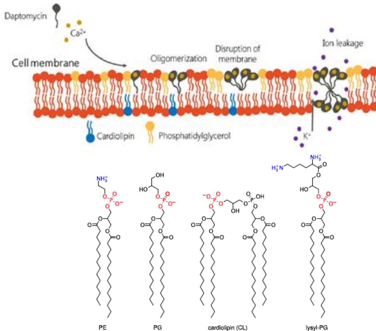
Figure 5. Major phospholipids of Gram-positive bacteria. Phosphatidylethanolamine (PE) is the major neutral phospholipid, whereas phosphatidylglycerol (PG) and cardiolipin (CL) are acidic; with CL, only one of the phosphate groups is usually deprotonated. Lysyl-PG carries a net positive charge. While the figure shows the myristoyl variants of all lipids, the fatty acyl residues in vivo are subject to variation in length and degree of unsaturation.
