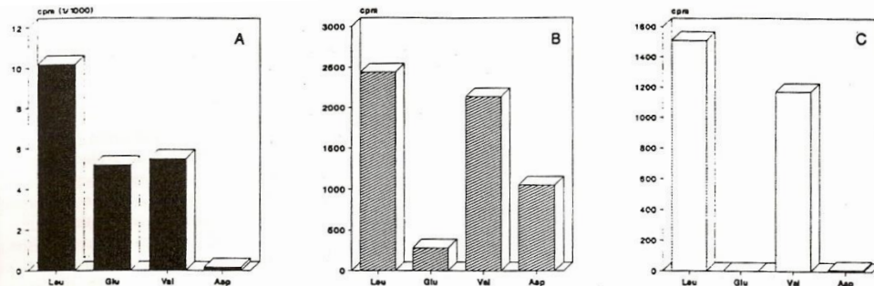
Fig. 5. Amino-acid binding activity of (A) srfAORF1, (B) srfAORF2 and (C) srfAORF3. Each enzyme subunit was incubated in the presence of ATP and one [ 14 C]-labelled amino acid. After 30 min incubation at 37°C, proteins were precipitated with 5% TCA, filtered through cellulose nitrate filters (MFS, USA) and the TCA precipitated material was counted.
