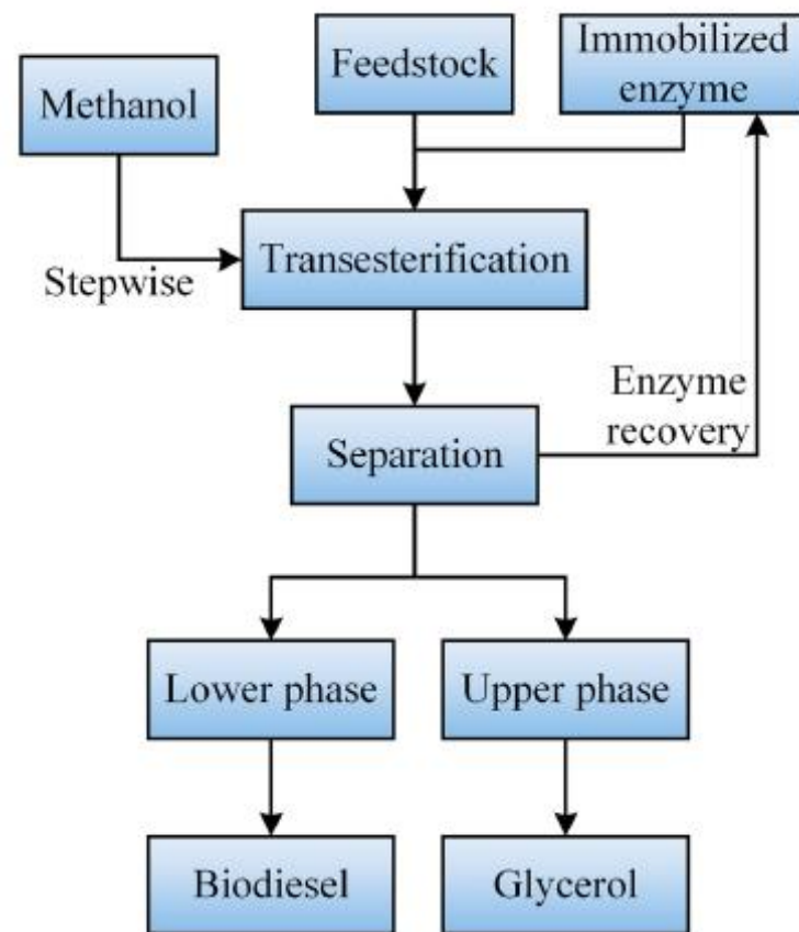
Fig. 10. Biodiesel production using enzymatic-catalyzed transesterification process.
