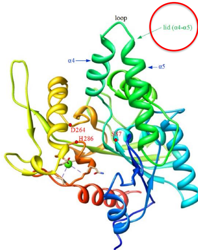
Figure 2. The structure of Burkholderia cepacia lipase: The lid region 118–159 (α4-loop-α5) and the catalytic triad (S87, D264, and H286) by red spheres are shown (Schrag et al., 1997).
