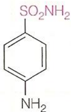
Sulfanilamide
