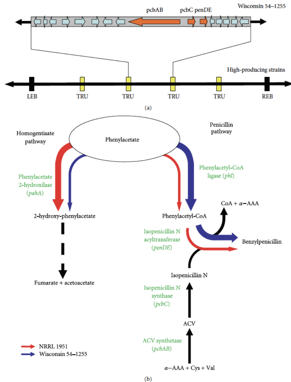
FIGURE 2: Examples of two well-known modifications that occurred during the strain improvement program. (a) Amplification of the DNA region containing the penicillin biosynthetic gene cluster in high-producing strains. LEB: left end border; REB: right end border; TRU: tandem repetition union. (b) Modification in the metabolic fluxes through the homogentisate pathway for phenylacetic acid catabolism and the penicillin biosynthetic pathway. Thickness of arrows indicates the flux rate through a specific enzyme. \alpha -AAA: \alpha -aminoadipic acid; ACV: \delta -(L- \alpha -aminoadipyl)-L-cysteinyl-D-valine; CoA: coenzyme A; Cys: cysteine; Val: Valine, Barreiro et al., 2011.
