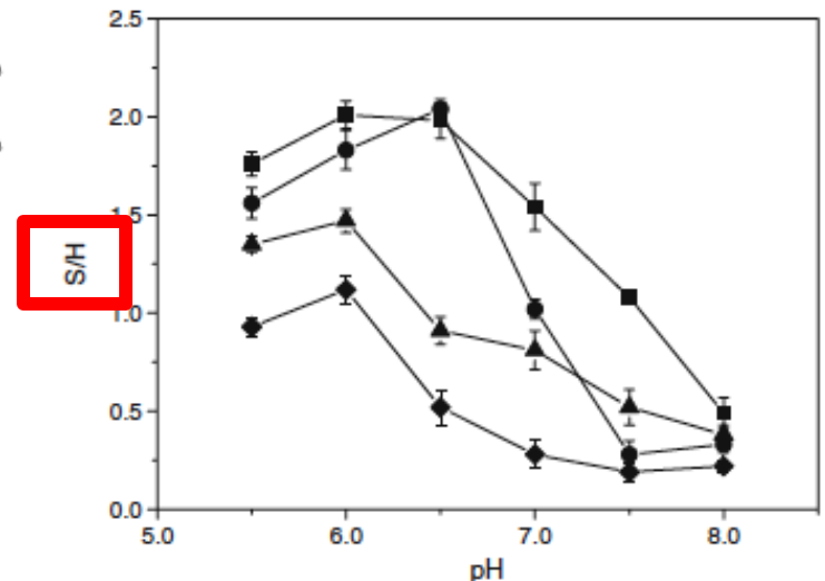
Fig. 4 Effect of pH on the S/H of the immobilized penicillin acylase. Square: AIPA; circle: KcPA; upright triangle: PCA; diamond: IPA
