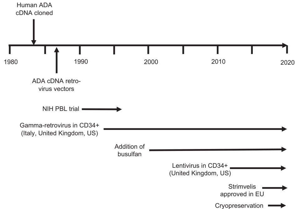
FIG 4. Timeline for development of HSC-GT for ADA deficiency. After identification and cloning of the cDNA for ADA, retroviral vectors were developed to efficiently deliver ADA. In 1990, the first gene therapy trial was initiated at the National Institutes of Health ( NIH ) by using patients' peripheral blood lymphocytes ( PBL ), followed by use of CD34 + hematopoietic stem cells. Since 2000, use of busulfan has been gradually incorporated into HSCT-GT, including lentivirus-based trials. In 2016, Strimvelis was approved for clinical use in the European Union ( EU ). Currently, the effect of cryopreservation of transduced cells is being explored.
