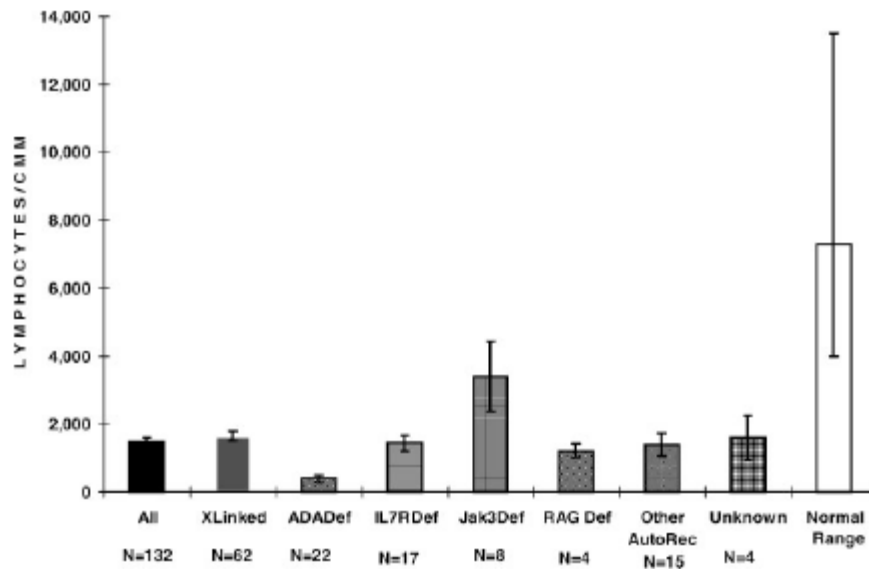
Figure 1 Means \pm SEM of absolute lymphocyte counts in 132 SCID infants at presentation, showing the characteristic of lymphopenia in all forms of SCID.
