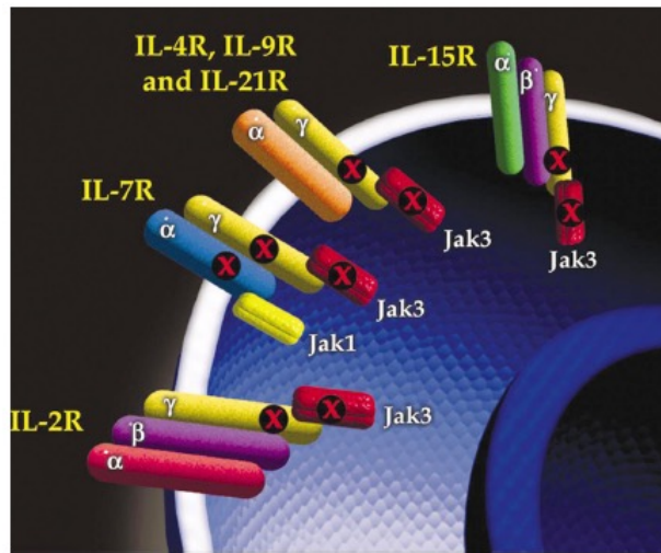
Figure 5 Diagram showing that Janus kinase 3 (Jak3) is the major signal transducer for the common gamma chain ( \gamma ) shared by multiple cytokine receptors. Mutations in the IL-2RG gene cause X-linked SCID, whereas mutations in the Jak3 gene result in a form of autosomal recessive SCID that mimics X-SCID in lymphocyte phenotype (i.e., T - B + NK - ). Mutations in the alpha chain of the IL-7 receptor also cause SCID, but unlike X-linked and Jak3-deficient SCID, IL-7R \alpha chain-deficient SCID infants have both B and NK cells (i.e., are T - B + NK + ). [Figure reprinted with permission from (27a).]
