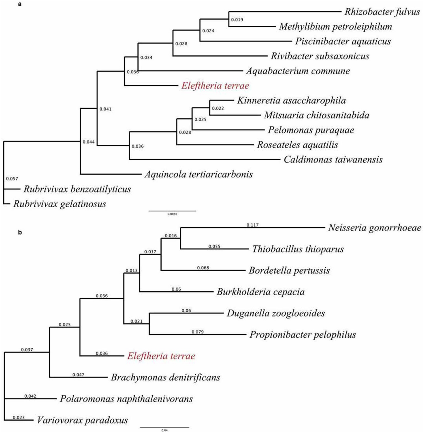
Extended Data Figure 2 | 16S rRNA gene phylogeny of Eleftheria terrae . a , The phylogenetic position of E. terrae within the class \beta -proteobacteria. The 16S rRNA gene sequences were downloaded from Entrez at NCBI using accession numbers retrieved from peer-reviewed publications. b , The phylogenetic position of E. terrae among its closest known relatives. The sequences were downloaded from NCBI using accession numbers retrieved from the RDP Classifier Database. For both trees, multiple sequence alignments (MSA) were constructed using ClustalW2, implementing a default Cost Matrix,
