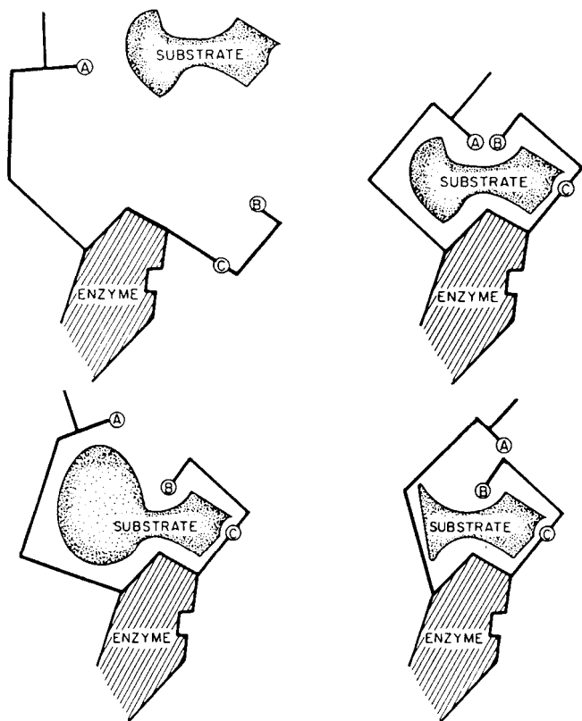
Fig.1. Schematic model of the induced fit mechanism. Black lines indicate protein chains containing catalytic groups A and B and binding group C. Upper left: substrate and enzyme dissociated. Upper right: substrate with induced change of protein chains to bring A and B into proper alignment for reaction. Lower left: bulky group added to substrate prevents proper alignment of A and B. Lower right: deletion of a group eliminates buttressing action on the chain containing A, so the thermodynamically stable complex has incorrect alignment of A and B.
