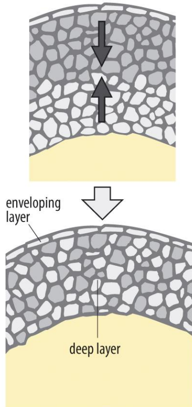
Radial intercalation
