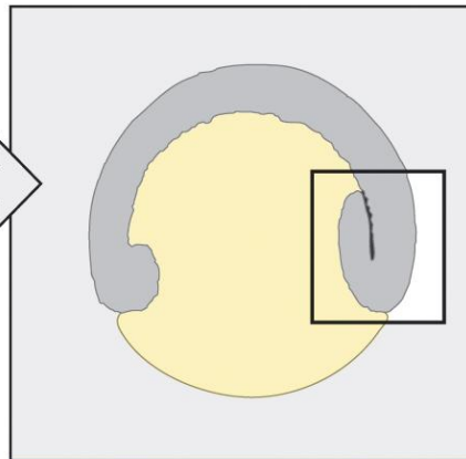
Epiboly
