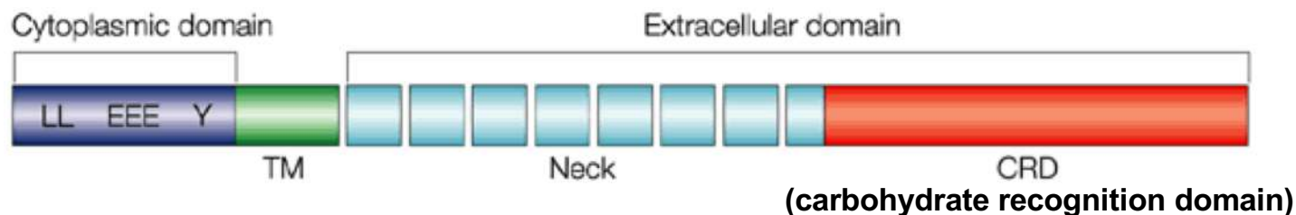
DC-SIGN binding site in the CRD
