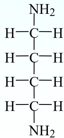
1,4-butandiammina ( putrescina )
