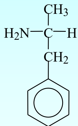
1-fenil-2-propanamina ( anfetamina )
