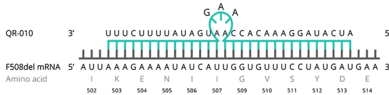
Fig. 6. Structure of the chemically modified QR-010 oligonucleotide used for mRNA repair. QR-010 is a single stranded, RNA oligonucleotide (33 nucleotides) with 2'O methyl base modifications and a phosphorothioate (PS) backbone to facilitate intracellular delivery and stability. QR-010 is designed to bind to sequences adjacent to the deleted F508 region in the CFTR mRNA resulting in the production of fully functional CFTR protein.
