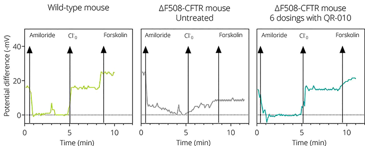
Fig. 7. Restoration of ion transport in nasal epithelium of F508del mice after treatment with QR-010. F508del mice were treated with six doses of QR-010, or remained untreated, and nasal potential difference (NPD) was measured. Representative NPD traces of wild-type, untreated, and QR-010-treated F508del mice are shown.
