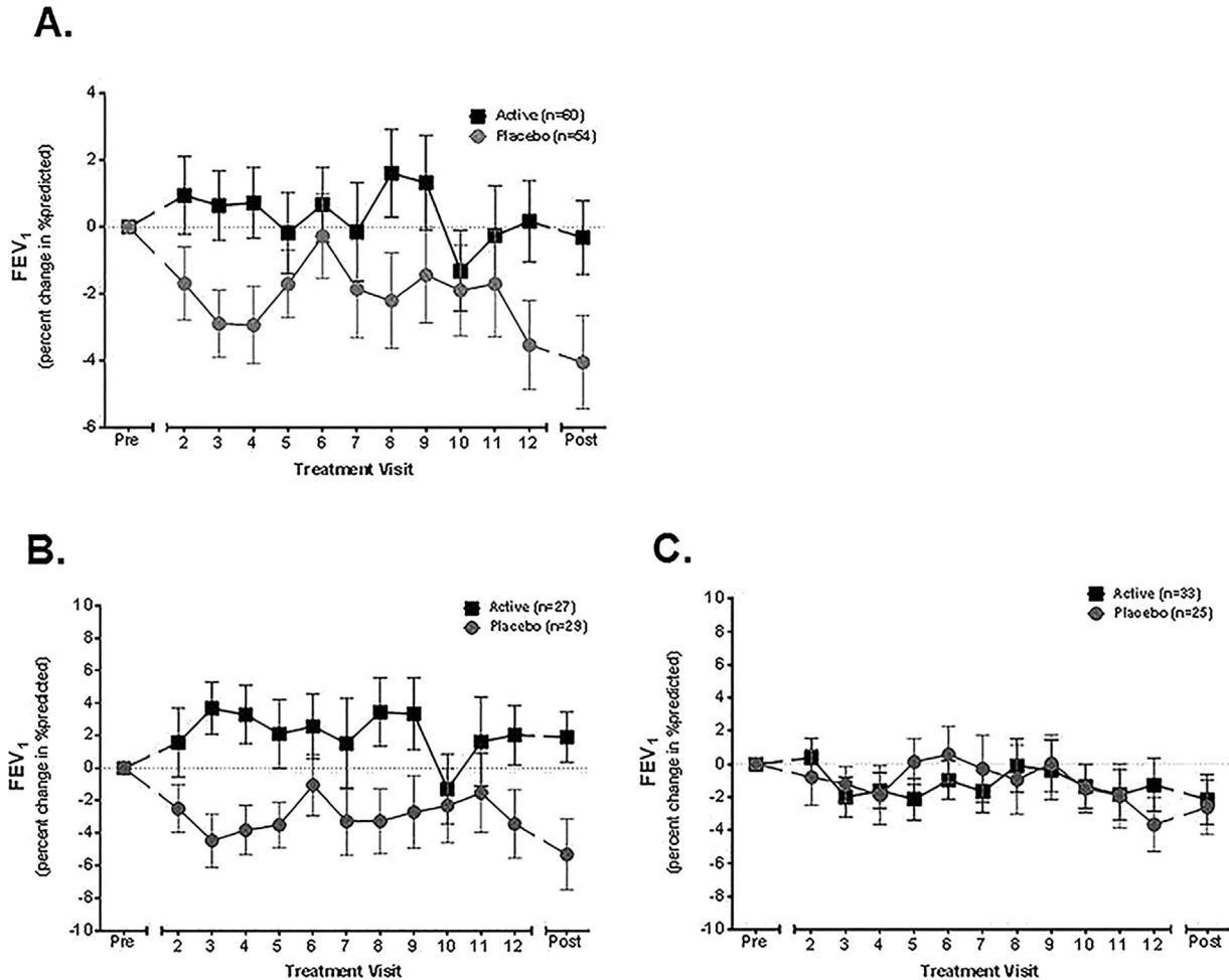
Fig. 2. Stabilization of lung function after repeated administration of the non-viral formulation pGM169/GL67A. Cystic fibrosis patients were treated monthly for 12 months with either active drug or the placebo. Lung function ( FEV_1 = forced expiratory volume in 1 sec) was measured at each treatment visit before administration of study drugs. Data are expressed as relative change from baseline in percent predicted FEV_1 . Error bars show the standard error of the mean. (A) All patients. There was a significant, albeit modest, treatment effect in the pGM169/GL67A group versus placebo at 12 months' follow-up (3.7%, P=0.046 ). (B) Patients with more severe lung function at start of treatment (Baseline FEV_1=50-70\% ), (C) Patients with less severe lung function at start of treatment (Baseline FEV_1=70-90\% ). The figure is adapted from Ref. 89 as part of a CCBY license.
