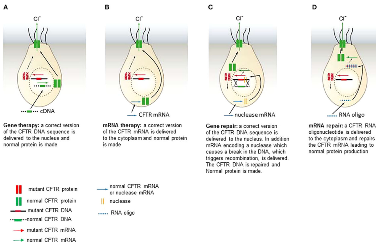
Fig. 1. Schematic presentation of “genetic medicine” strategies that are currently being developed for CF. The basic concepts of gene therapy (A) and mRNA therapy (B), as well as gene editing (C) and mRNA repair (D) are outlined. In addition to chloride ( \text{Cl}^- ) ions, CFTR also conducts a number of other anions, including bicarbonate. For simplicity these molecules are not shown in the figure.
