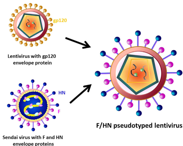
Fig. 3. Generation of F/HN-pseudotyped lentiviral vector. Molecular techniques enable the replacement of the gp120 envelope glycoprotein, which supports lentivirus entry into T-cells but is not suitable for entry into airway epithelial cells, with the F (fusion) and HN (hemagglutinin-neuraminidase) proteins from Sendai virus which support efficient entry into airway epithelial cells. This process of pseudotyping leads to the generation of a chimeric pseudotyped F/HN lentiviral vector. The Sendai virus F and HN proteins were chosen because they are, in part, responsible for the high transduction efficiency of Sendai virus in lungs. 8
