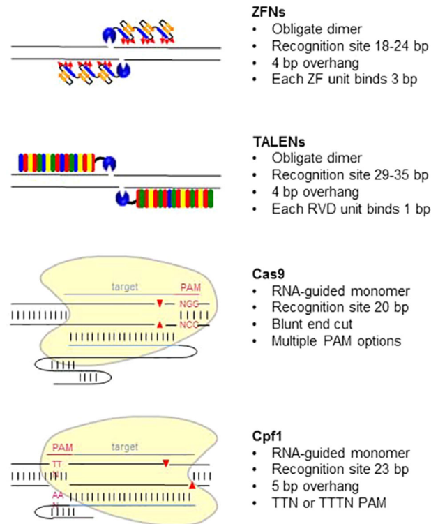
Fig. 5. Programmable and RNA-guided DNA endonucleases. Schematic representation of the four most commonly used programmable and RNA-guided DNA endonucleases. ZNF, zinc finger nucleases; ZF, zinc finger; TALEN, TAL-effector nucleases; PAM, protospacer adjacent motif; RVD, repeat variable di-residue.
