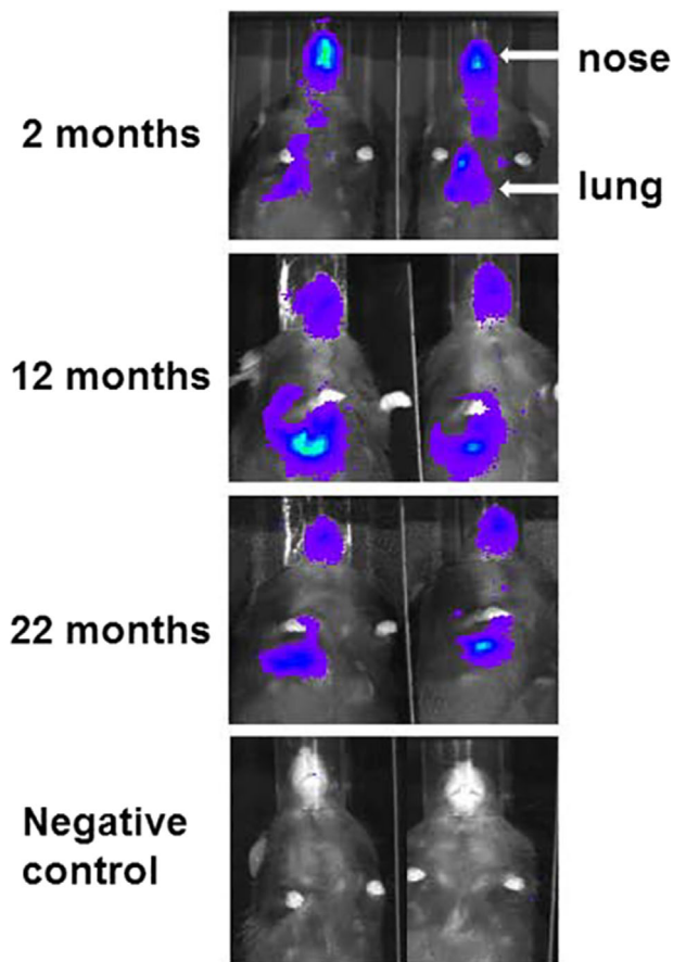
Fig. 4. F/HN-pseudotyped lentivirus transduction leads to persistent gene expression in mouse airways. Mice were transduced with F/HN-pseudotyped lentivirus expressing a luciferase reporter gene by nasal sniffing (or received PBS (negative controls). Luciferase expression was visualized using bioluminescence imaging, 2–22 months after transduction.
