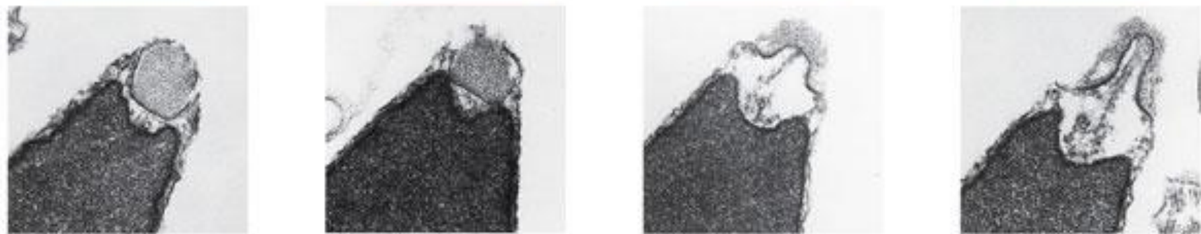
DEVELOPMENTAL BIOLOGY 11e , Figure 7.10
