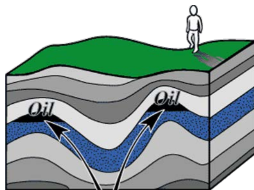
Anticline Traps
