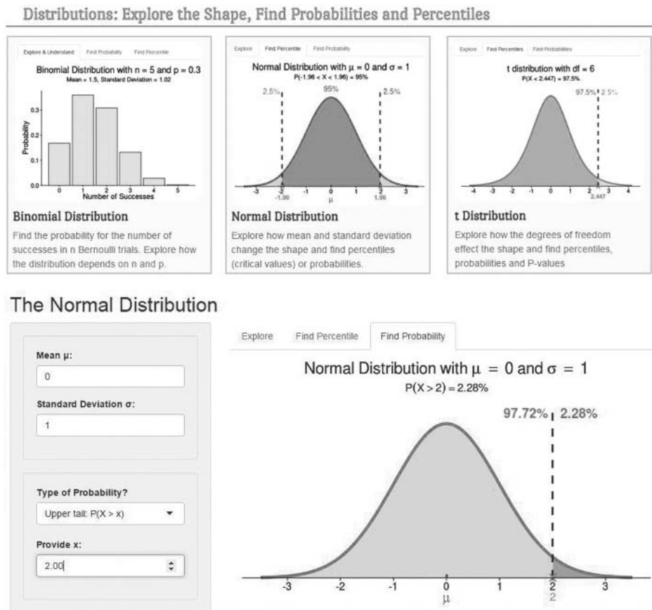
FIGURE 4.5: Go to www.artofstat.com/webapps.html for Useful Internet Applets. For normal probabilities, click on Normal Distribution . The applet denotes a variable by X and a possible value by x . Tail probabilities do not depend on values entered for \mu and \sigma .
