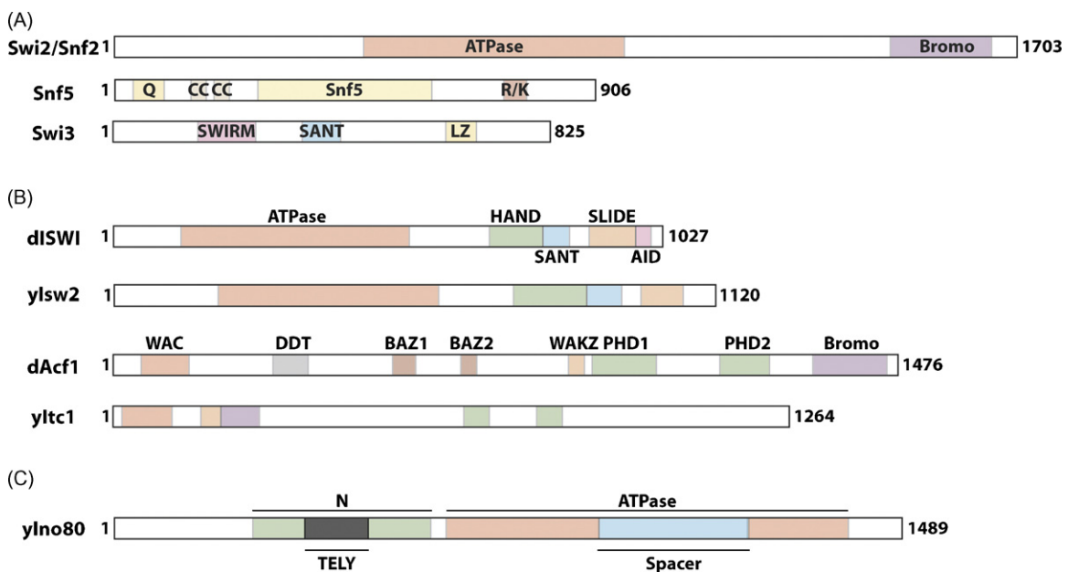
Fig. 3. Domain organization of the various subunits of different chromatin remodeling complexes. (A) The domains that have been found in three of the SWI/SNF subunits, namely Snf2, Snf5, and Swi3. (B) The catalytic subunit of the ISWI complexes from yeast and flies are compared, as well as that of the large accessory subunit of CHRAC/ACF and ISW2. (C) The domain organization of the catalytic subunit of the INO80 complex is shown. The abbreviations for the different domains are bromo for bromodomain, 'Q' represents the Q rich region, 'CC' for coiled coil region, 'R/K' for Arginine/Lysine rich basic region, and 'LZ' for Leucine Zipper.
