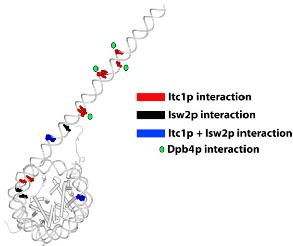
Fig. 4. Nucleosome interactions by ISW2. ISW2 interacts at three distinct sites on the nucleosome – extranucleosomal DNA, 10 bp into entry/exit site and two helical turns away from the dyad axis (SHL-2) [130]. Itc1p interacts predominantly with the extranucleosomal DNA and is represented in red. Isw2p interacts with extranucleosomal DNA close to the entry/exit site and near SHL2 and is represented in black. Regions where both Isw2p and Itc1p are present are represented in blue. Dpb4p interaction is restricted to the extranucleosomal DNA and is represented by green circles.
