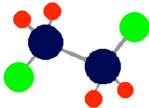
1,2-dichloroethane
