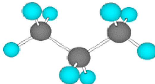
propano ( C_3H_8 )
